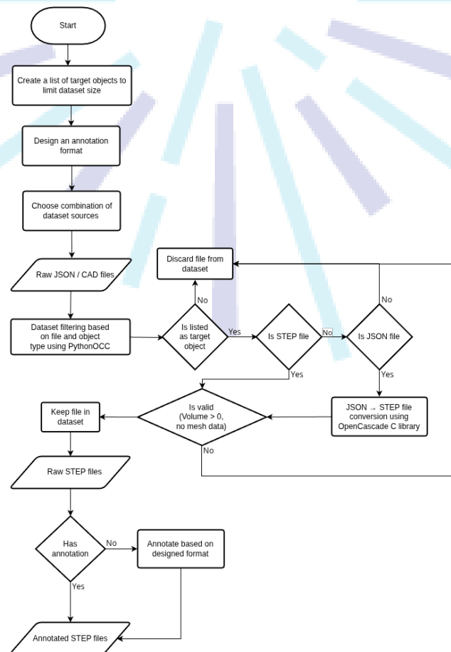
Figure 4 Dataset acquisition and filtering flowchart
